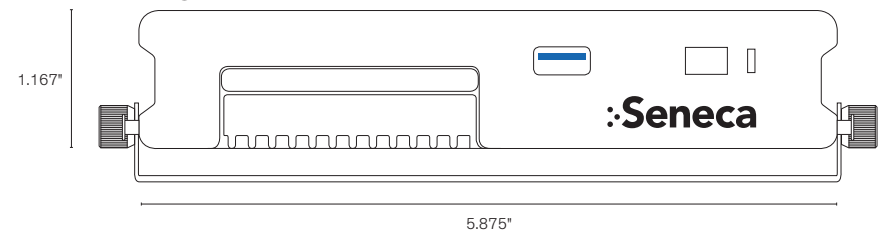
FRONT
